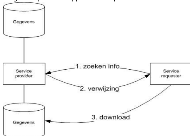
Figuur B1. Use case 'Download'
